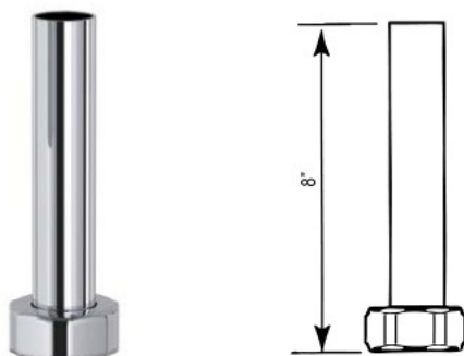
Raccord d'alimentation 8" 8" Thermostatic Outlet Connector
