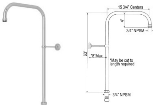
Raccord d'alimentation 8" 8" Thermostatic Outlet Connector
