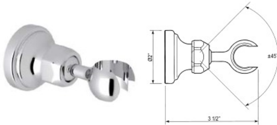
Support de douchette mural Wall Mount Handshower Holder
